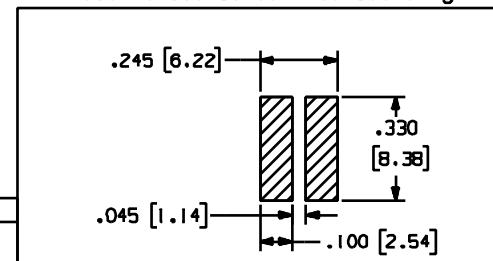
Recommended Solder Pad Geometry
