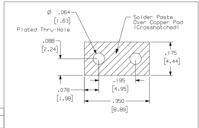
Recommended Solder Pad Geometry
