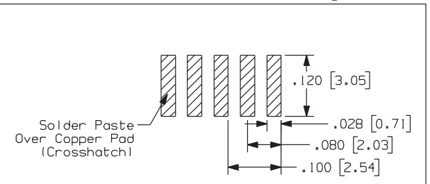
Alternate Solder Pad Geometry
