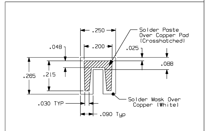
Recommended Solder Pad Geometry
